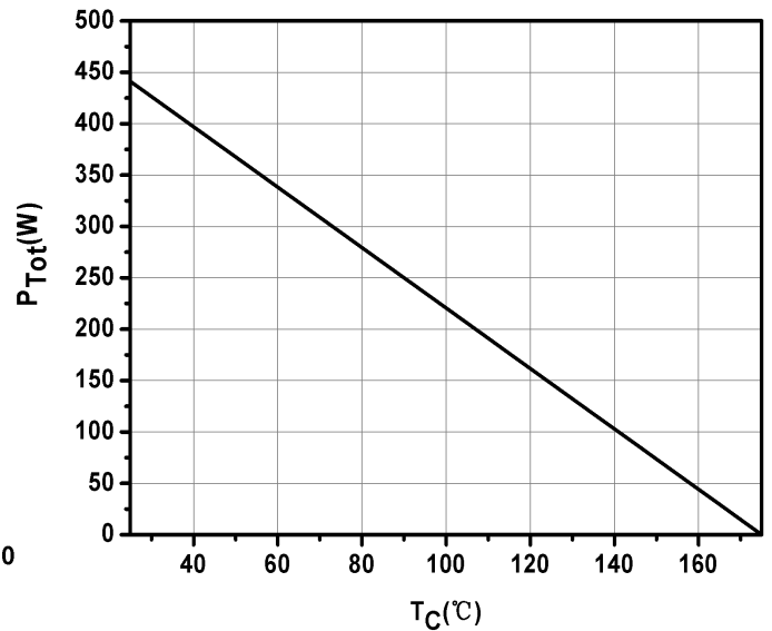
Fig.6-Power Derating
